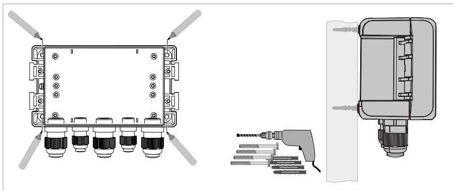
Figure 3-3: Wall mounting of the plastic housing
